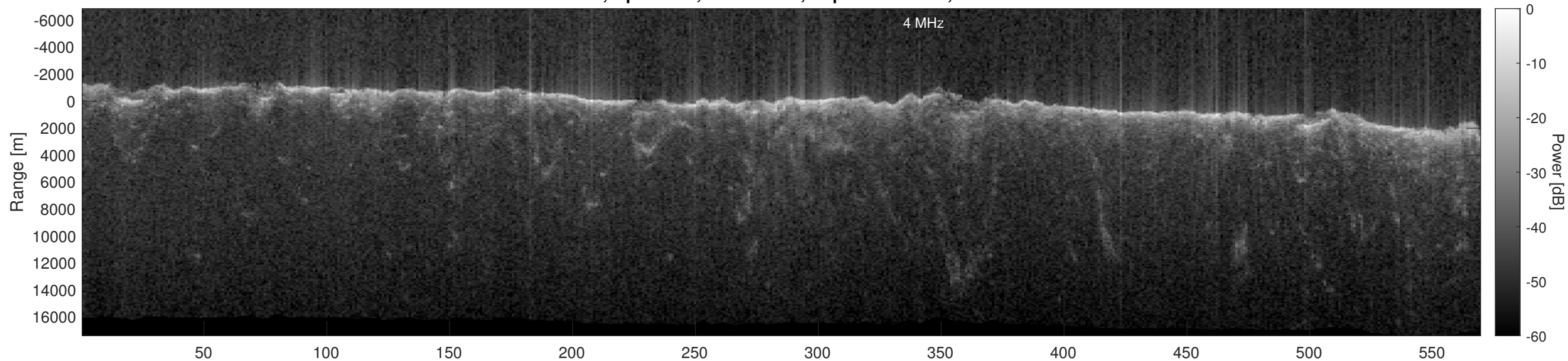
Orbit 6161, Optimized, No Window, Depth-Corrected, Channel 2
