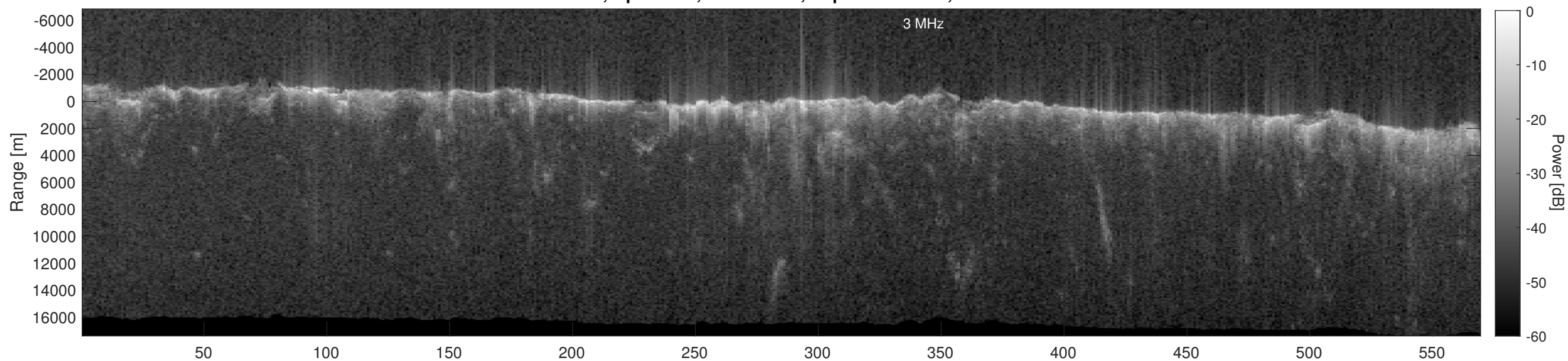
Orbit 6161, Depth-Corrected Cluttergram
