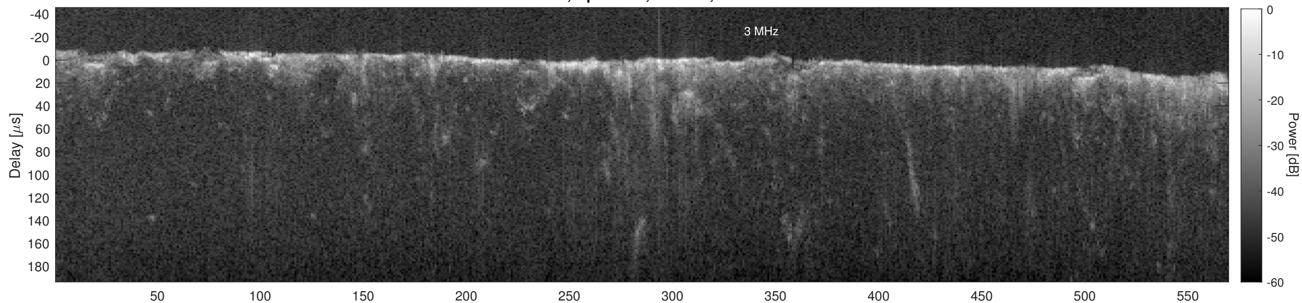
Orbit 6161, Cluttergram
