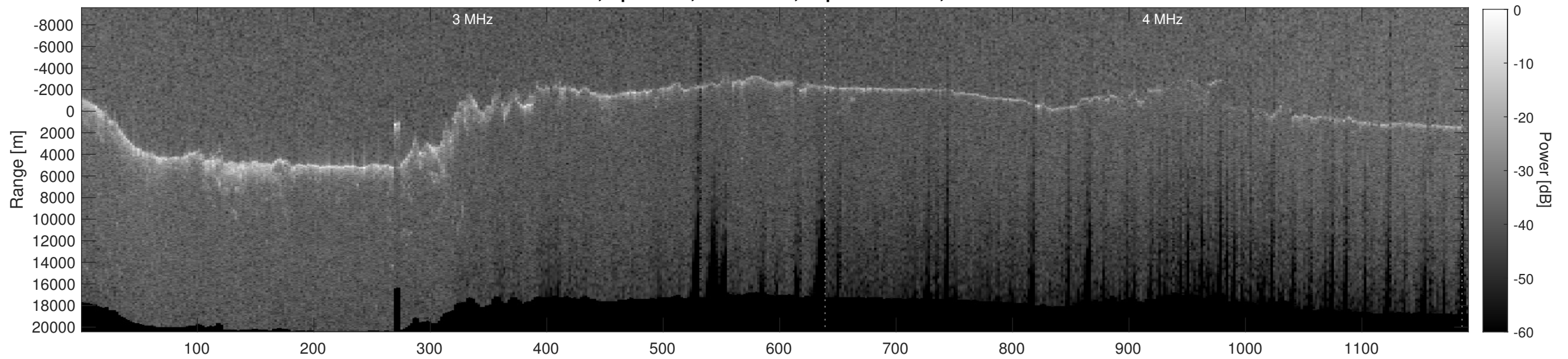
Orbit 6164, Depth-Corrected Cluttergram
