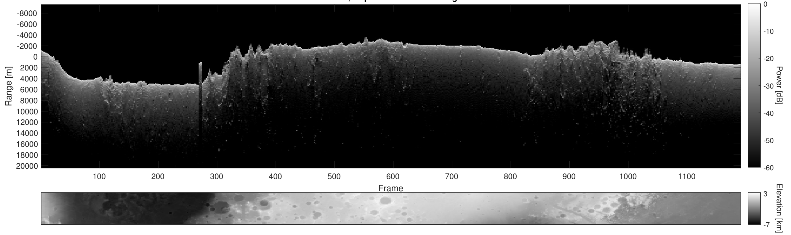
Orbit 6164, Depth-Corrected Cluttergram
