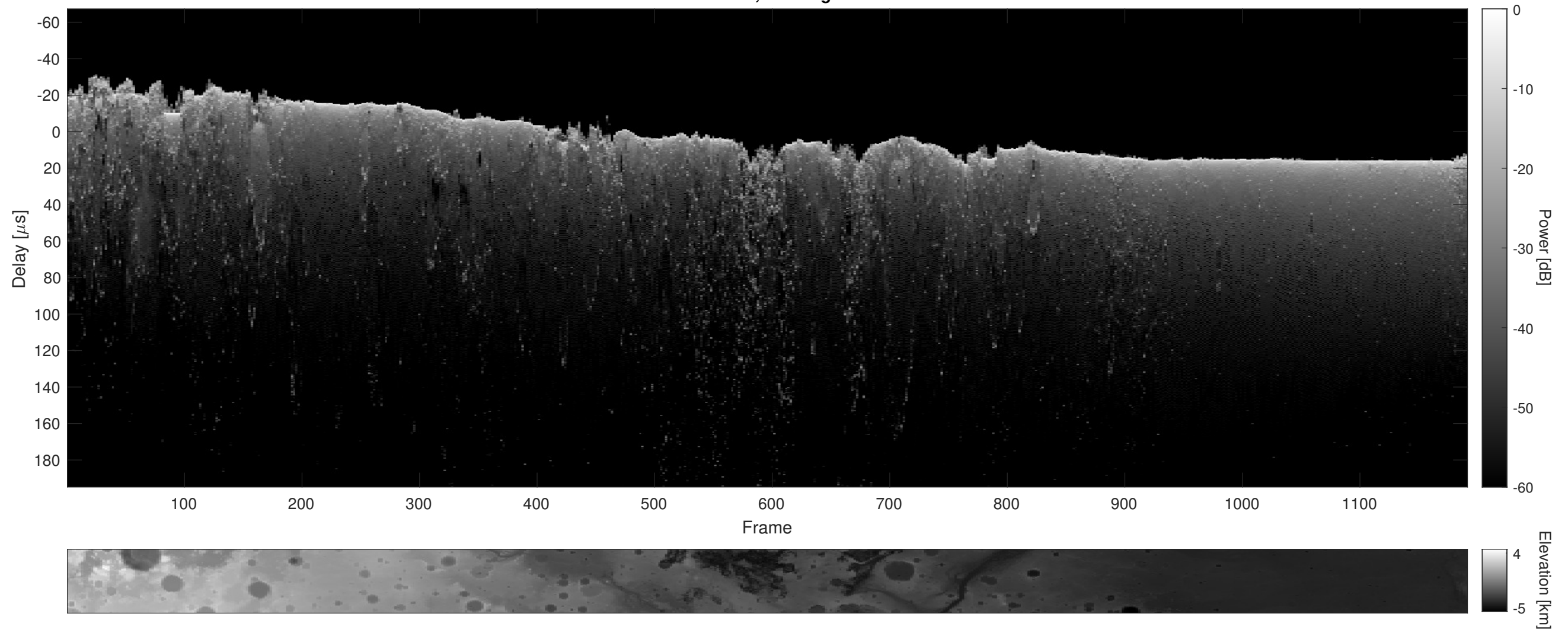
Orbit 6165, Cluttergram
