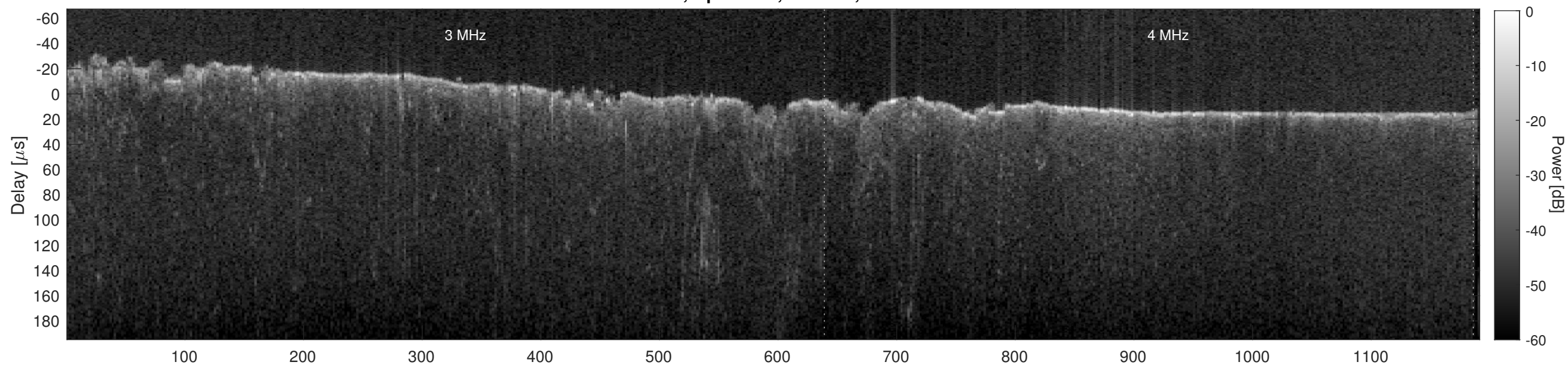
Orbit 6165, Cluttergram
