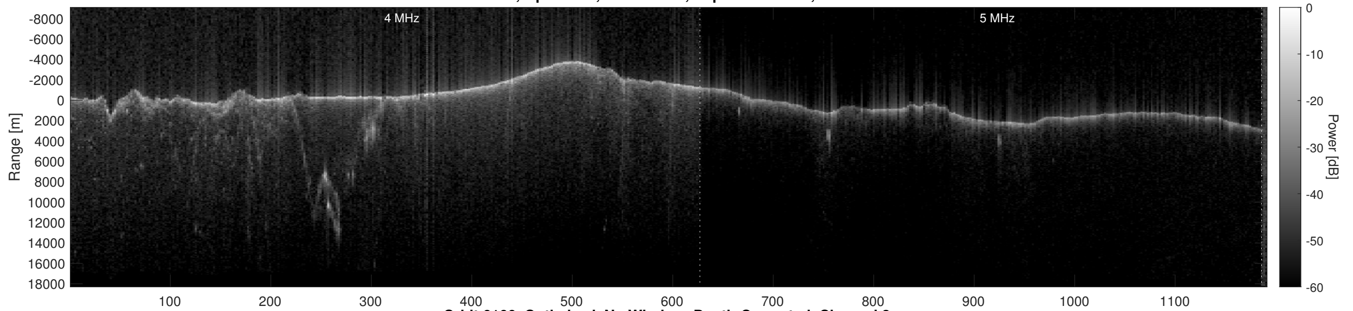
Orbit 6166, Optimized, No Window, Depth-Corrected, Channel 2
