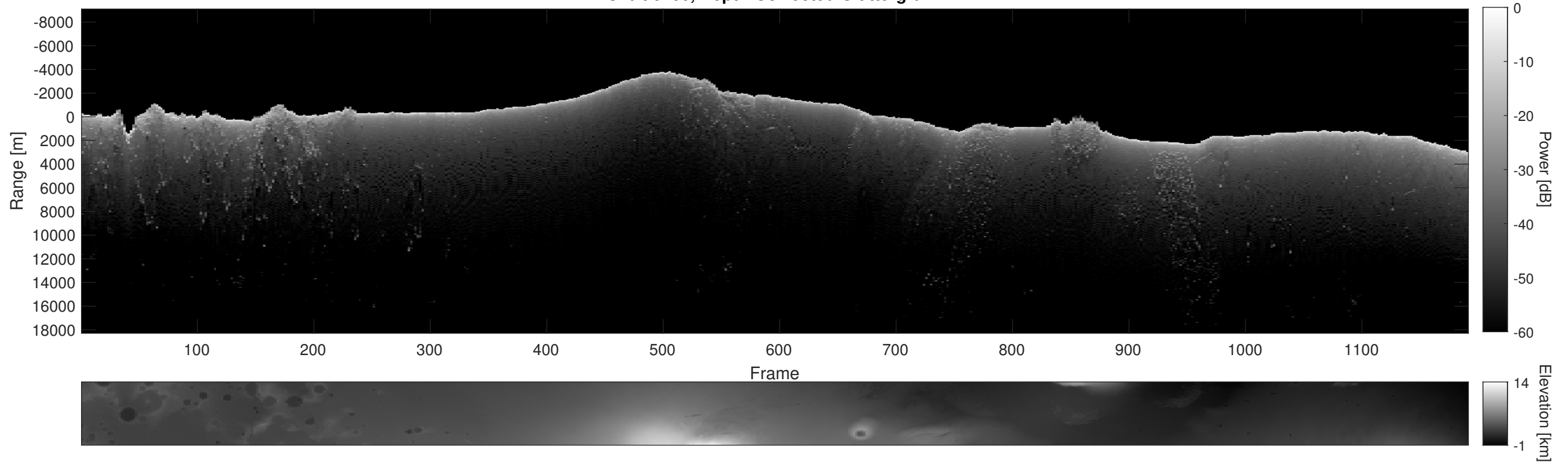
Orbit 6166, Depth-Corrected Cluttergram
