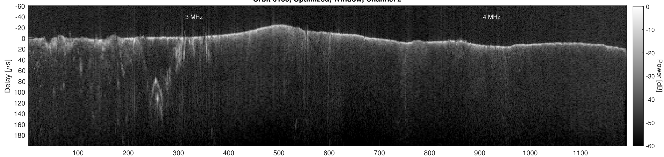
Orbit 6166, Cluttergram
