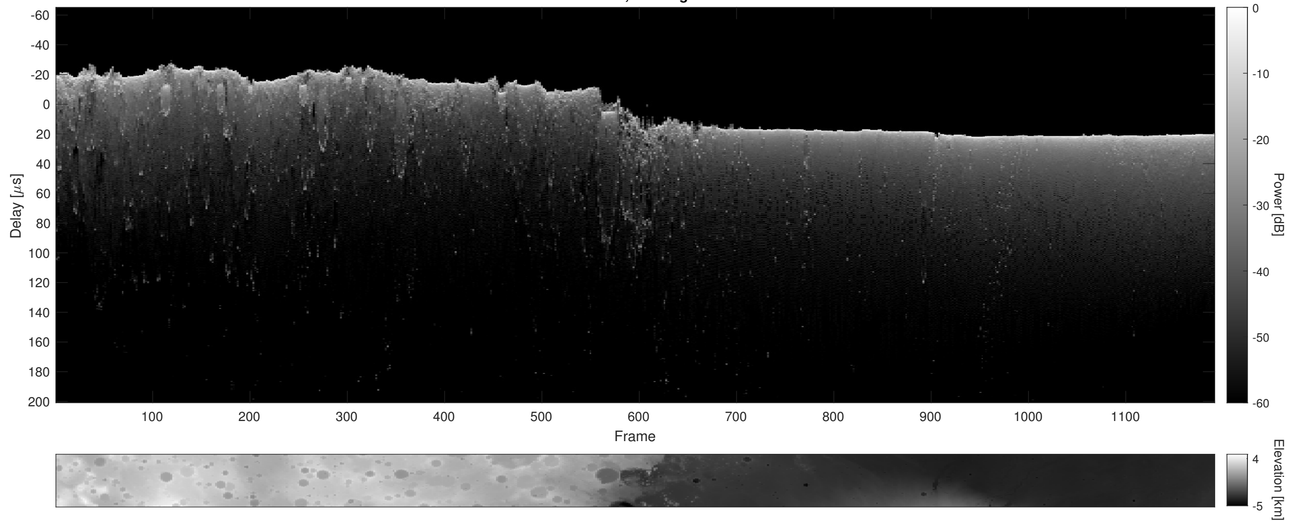
Orbit 6167, Cluttergram
