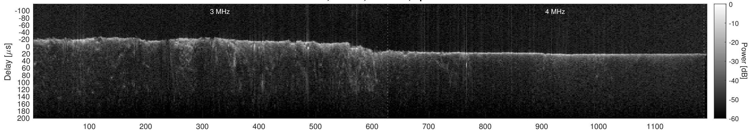
Orbit 6167, Cluttergram
