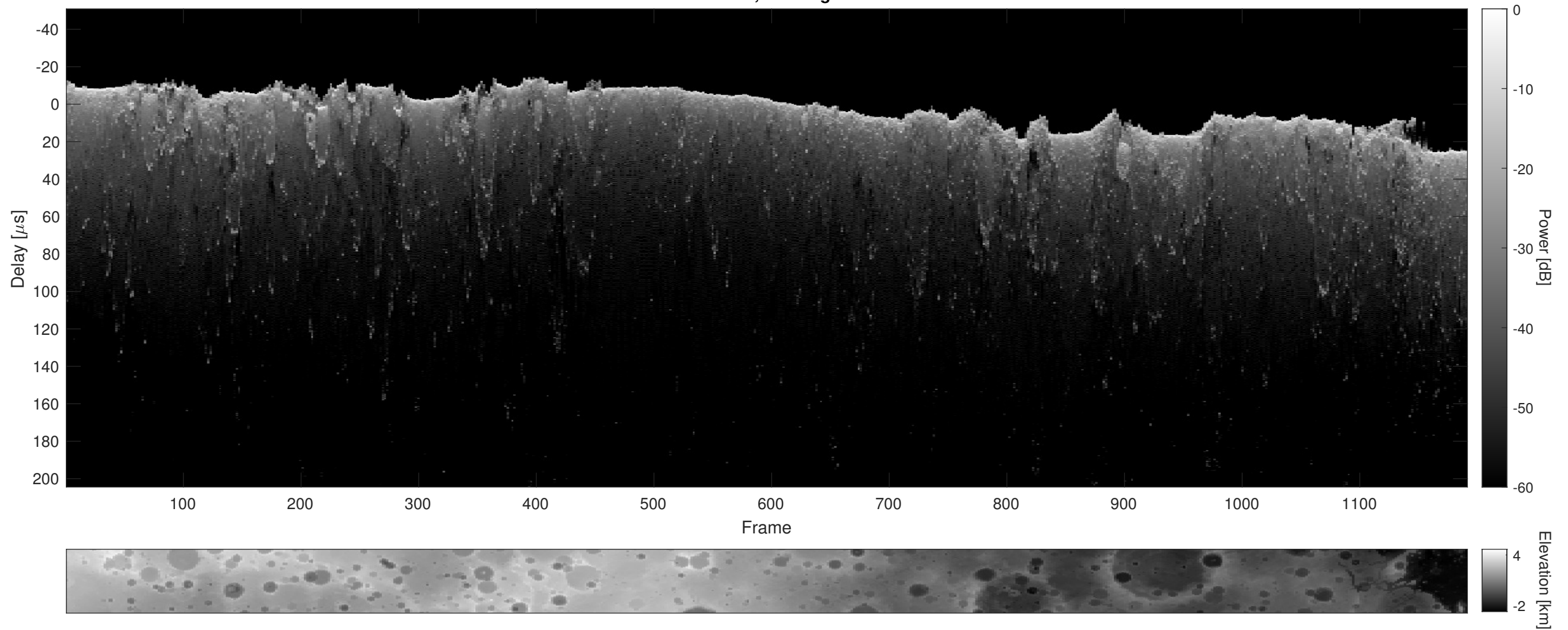
Orbit 6168, Cluttergram
