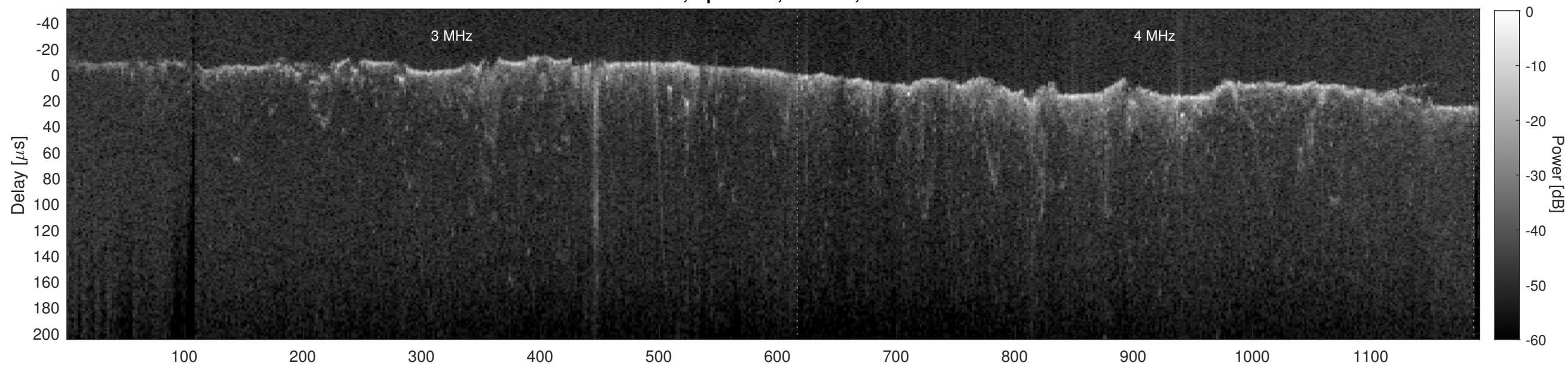
Orbit 6168, Cluttergram
