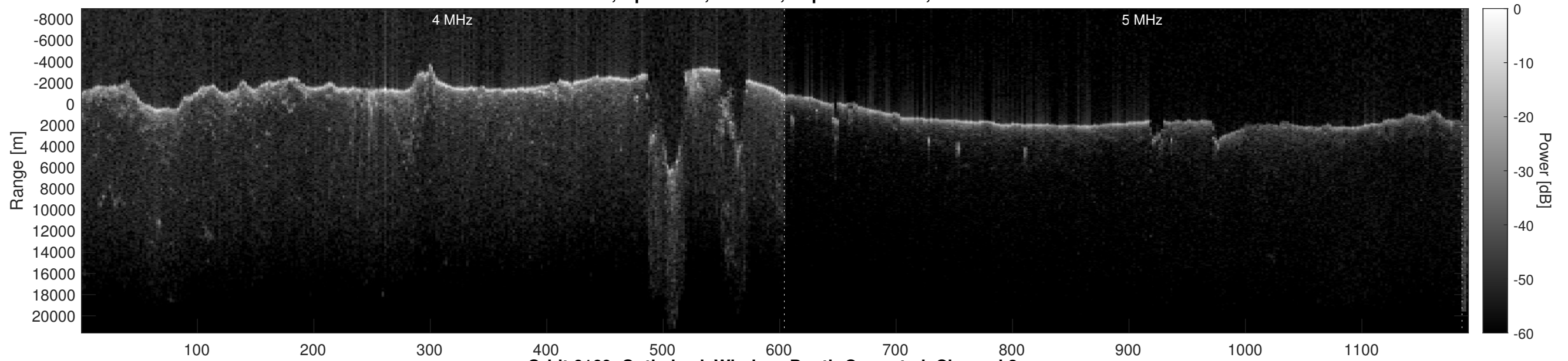
Orbit 6169, Optimized, Window, Depth-Corrected, Channel 2
