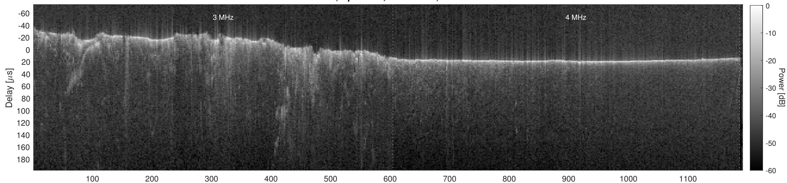
Orbit 6170, Cluttergram
