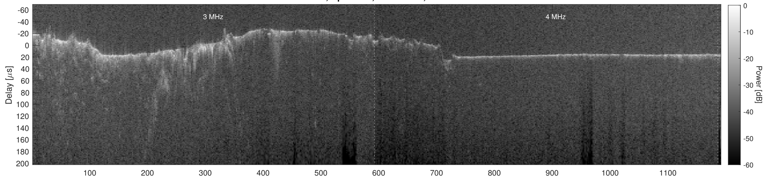
Orbit 6171, Cluttergram
