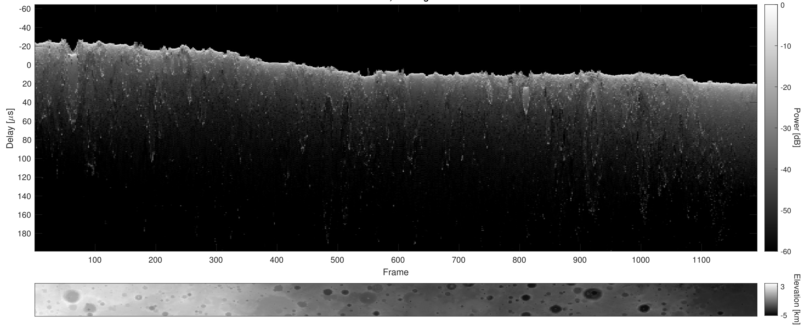
Orbit 6172, Cluttergram
