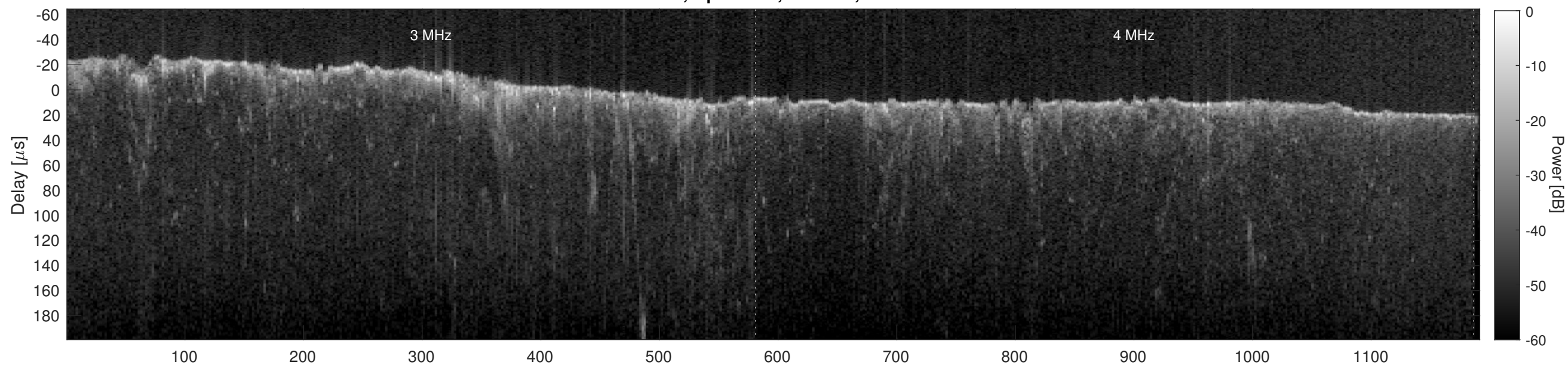
Orbit 6172, Cluttergram
