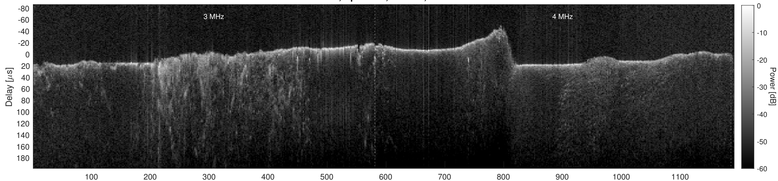
Orbit 6173, Cluttergram
