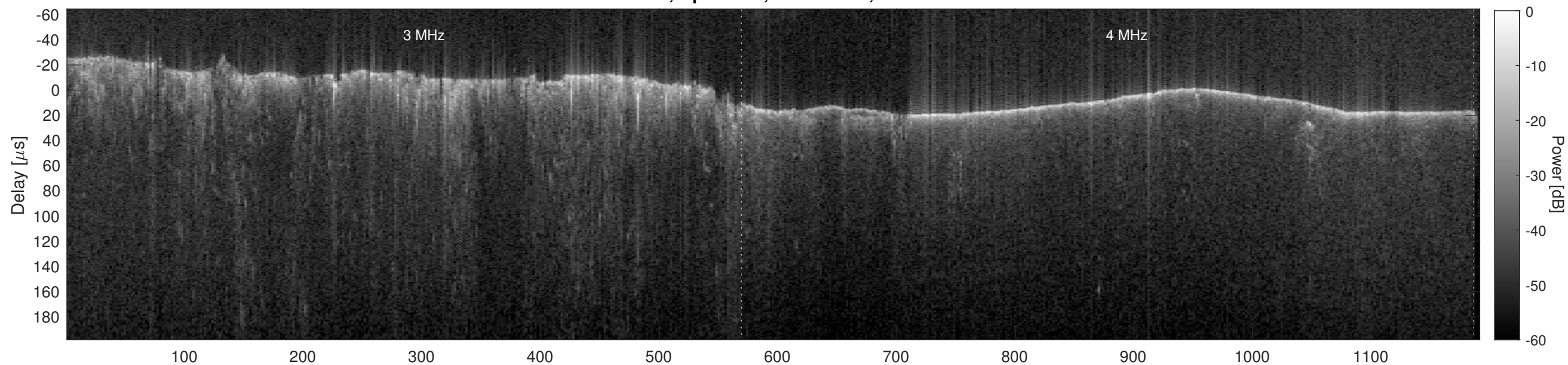
Orbit 6174, Cluttergram
