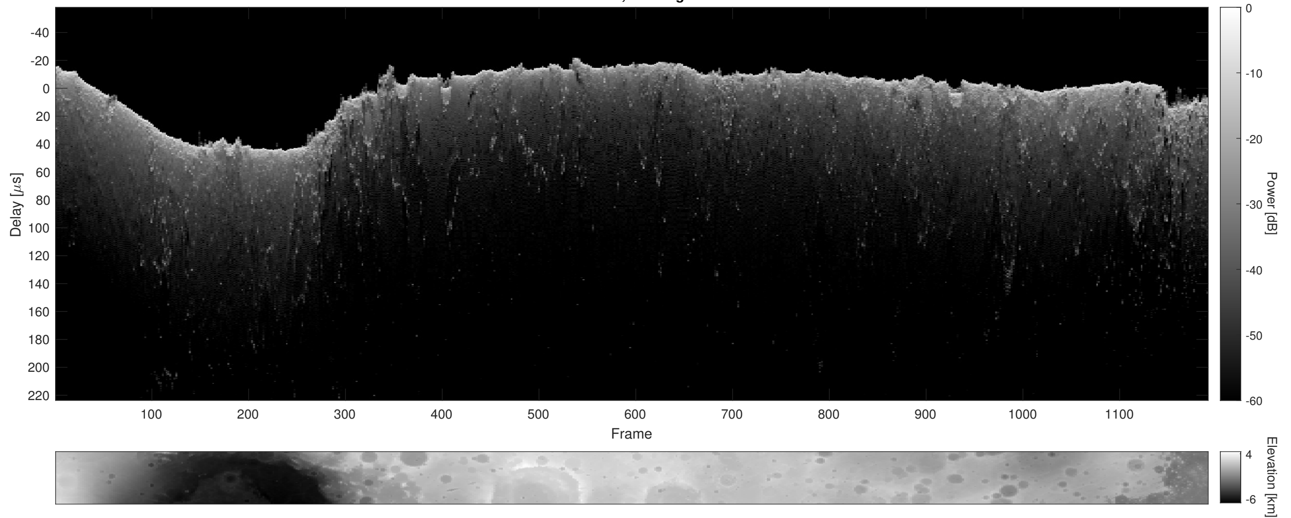
Orbit 6175, Cluttergram
