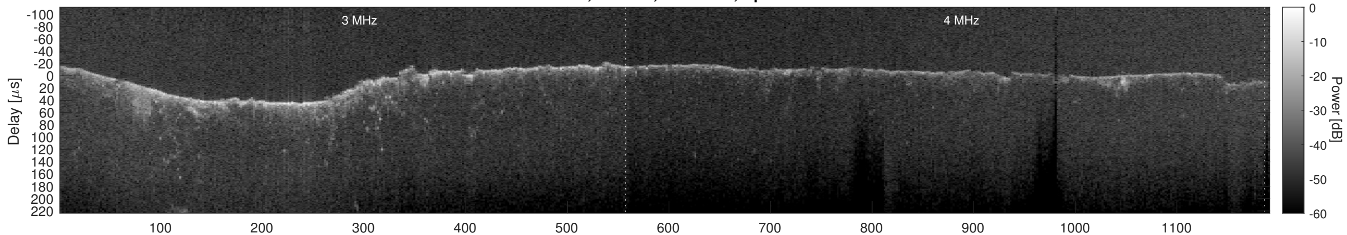
Orbit 6175, Cluttergram
