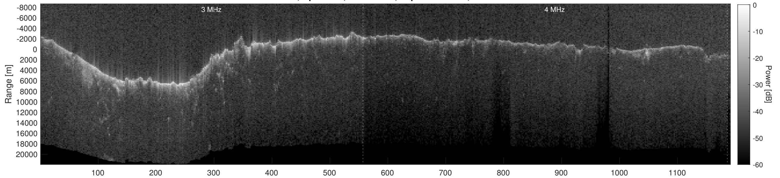
Orbit 6175, Depth-Corrected Cluttergram
