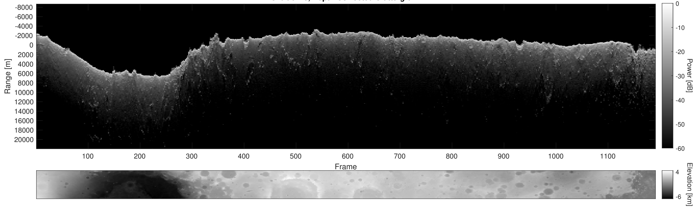
Orbit 6175, Depth-Corrected Cluttergram
