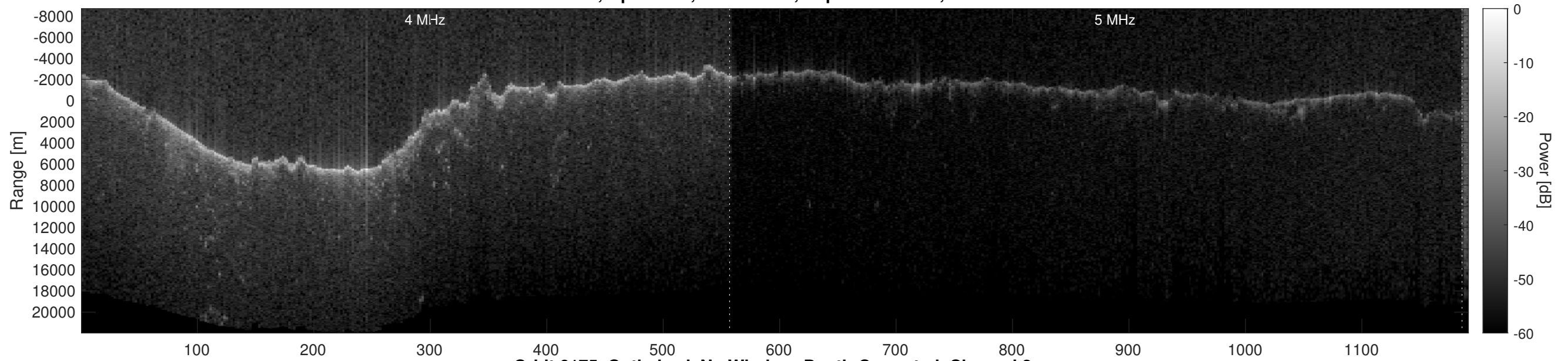
Orbit 6175, Optimized, No Window, Depth-Corrected, Channel 2
