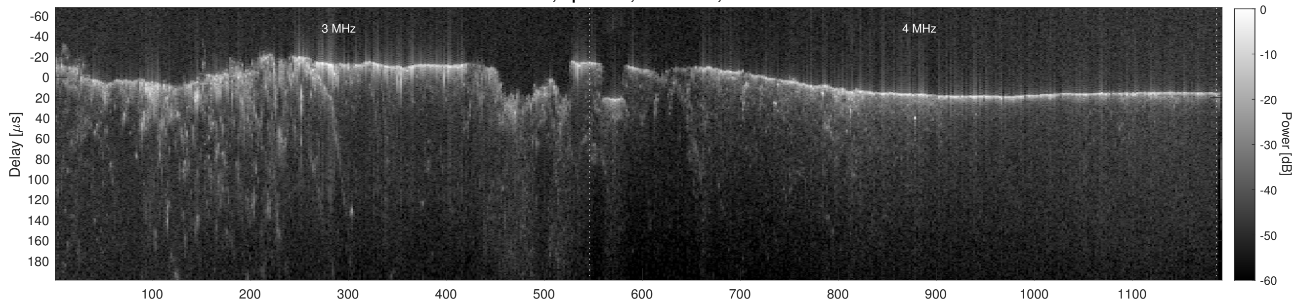
Orbit 6176, Cluttergram
