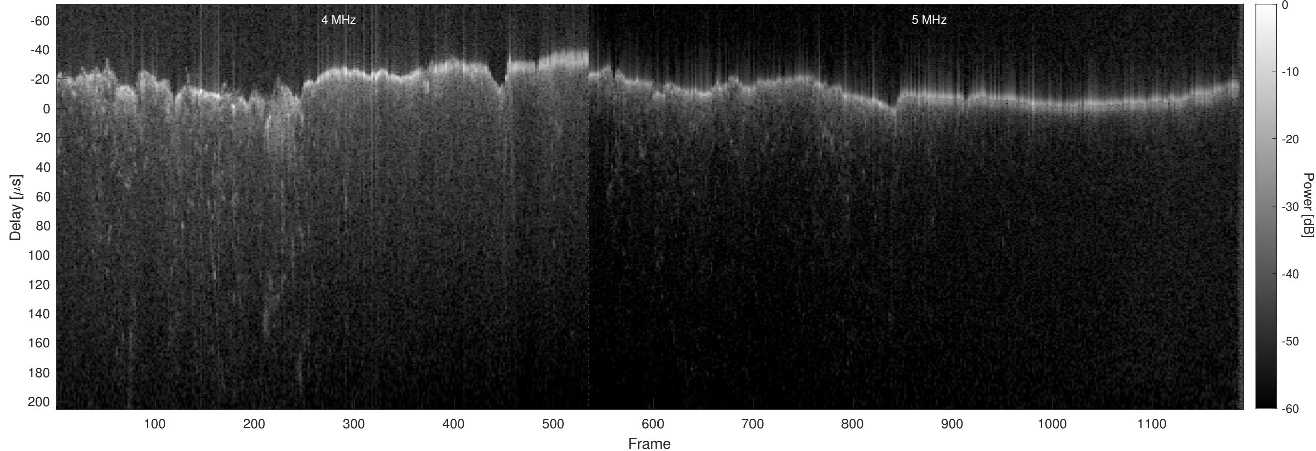
Orbit 6178, Chapman, No Window, Channel 2
