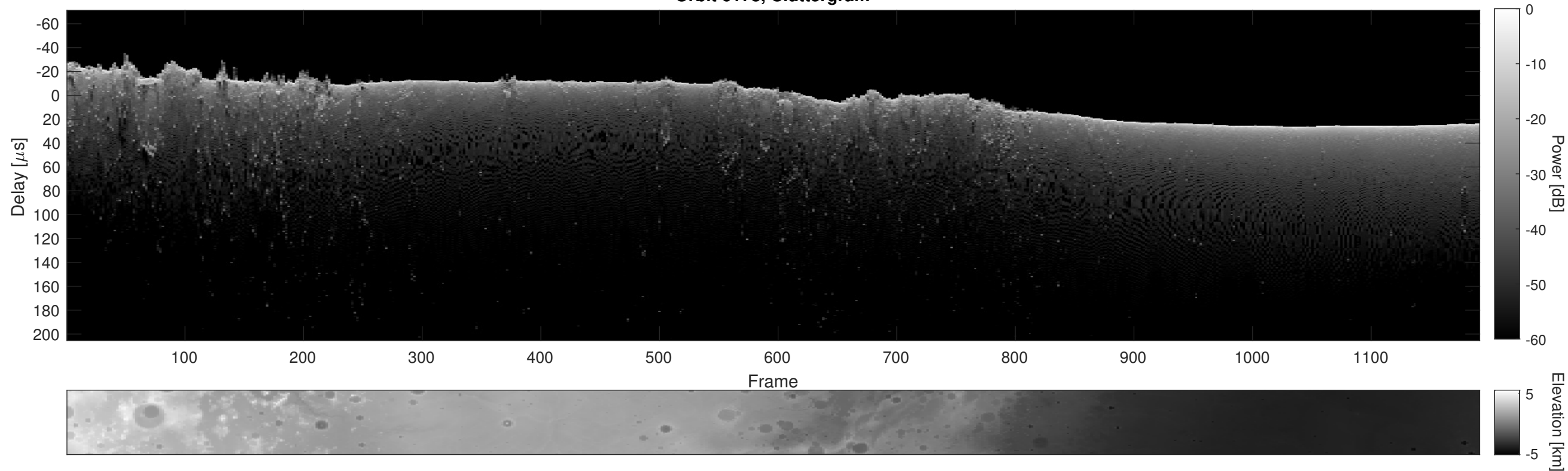
Orbit 6178, Cluttergram
