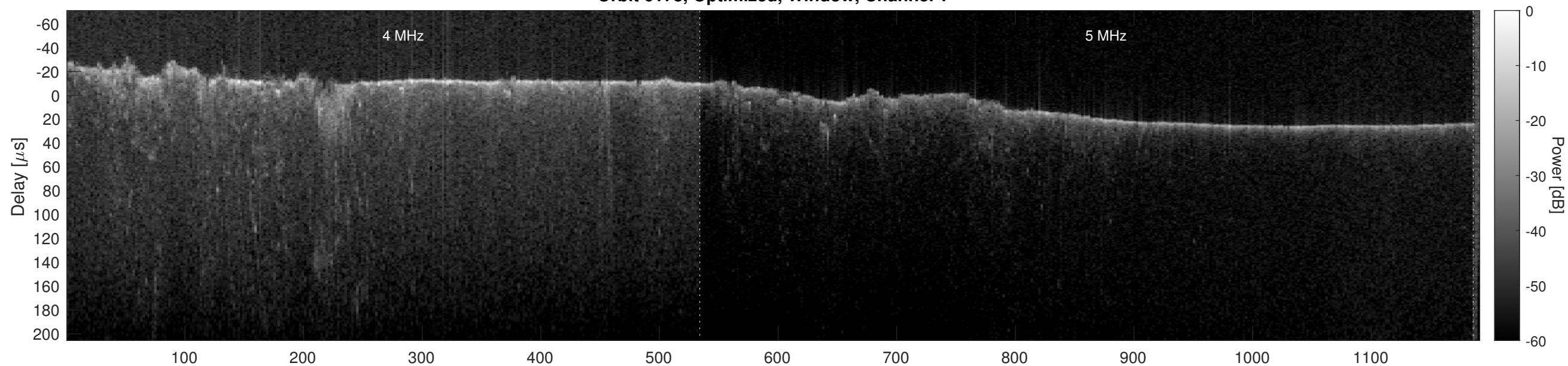
Orbit 6178, Optimized, Window, Channel 2
