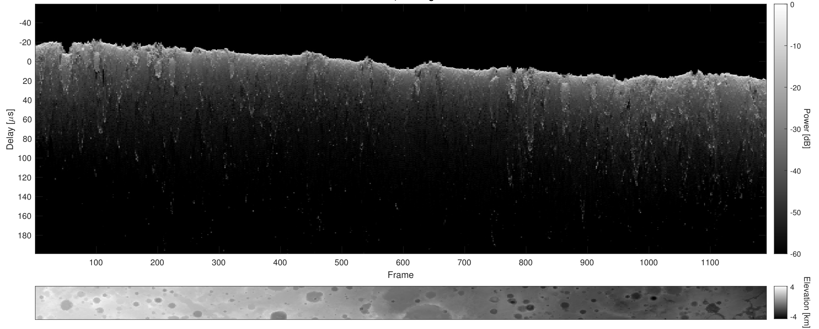
Orbit 6179, Cluttergram
