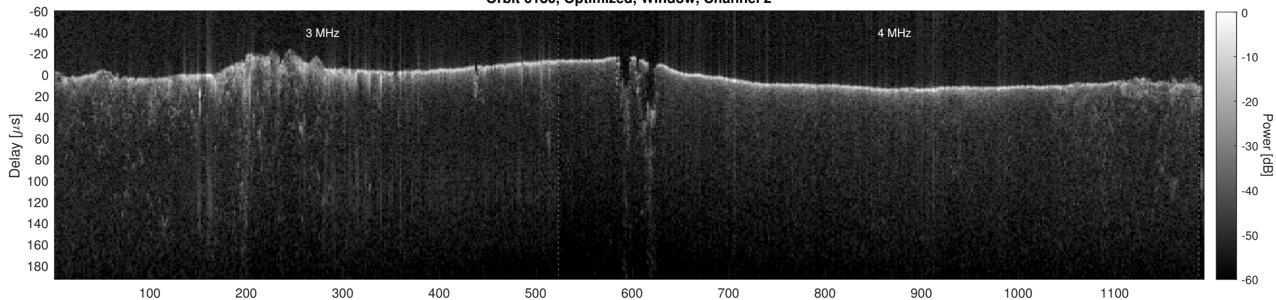
Orbit 6180, Cluttergram
