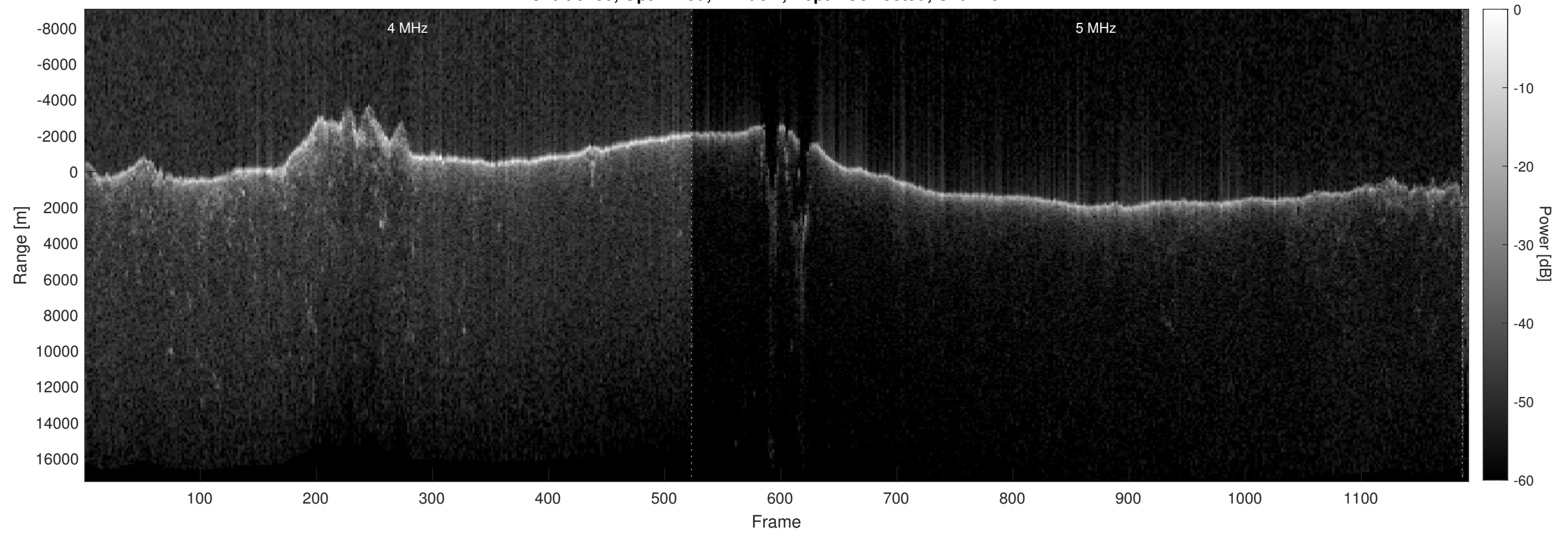
Orbit 6180, Optimized, Window, Depth-Corrected, Channel 2
