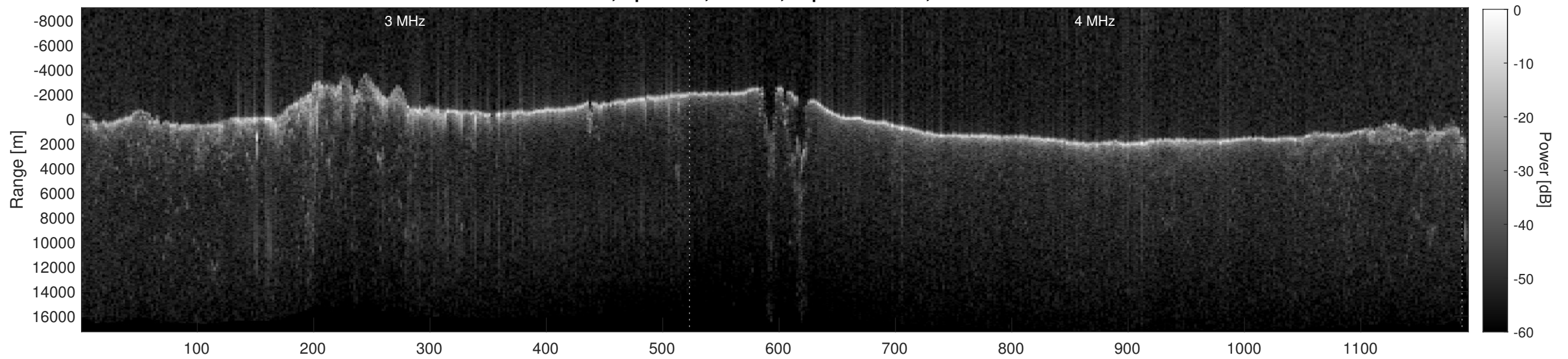
Orbit 6180, Depth-Corrected Cluttergram
