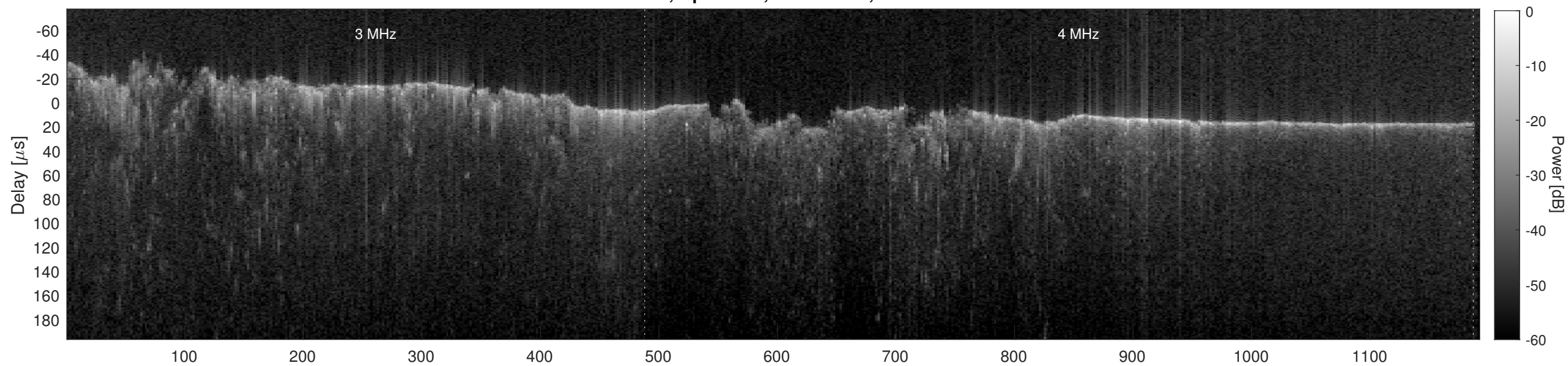
Orbit 6183, Cluttergram
