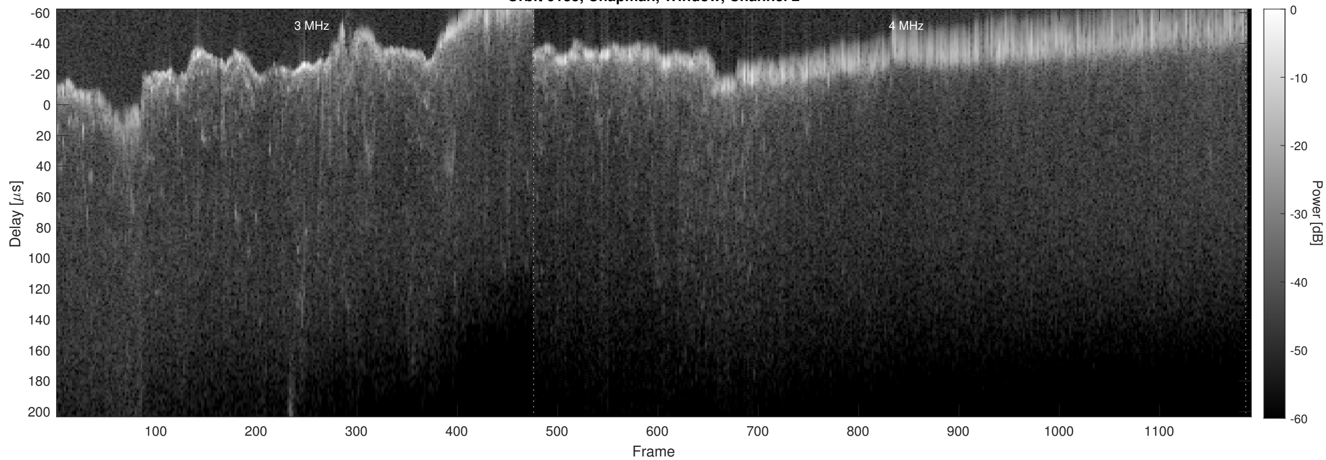
Orbit 6185, Chapman, Window, Channel 2
