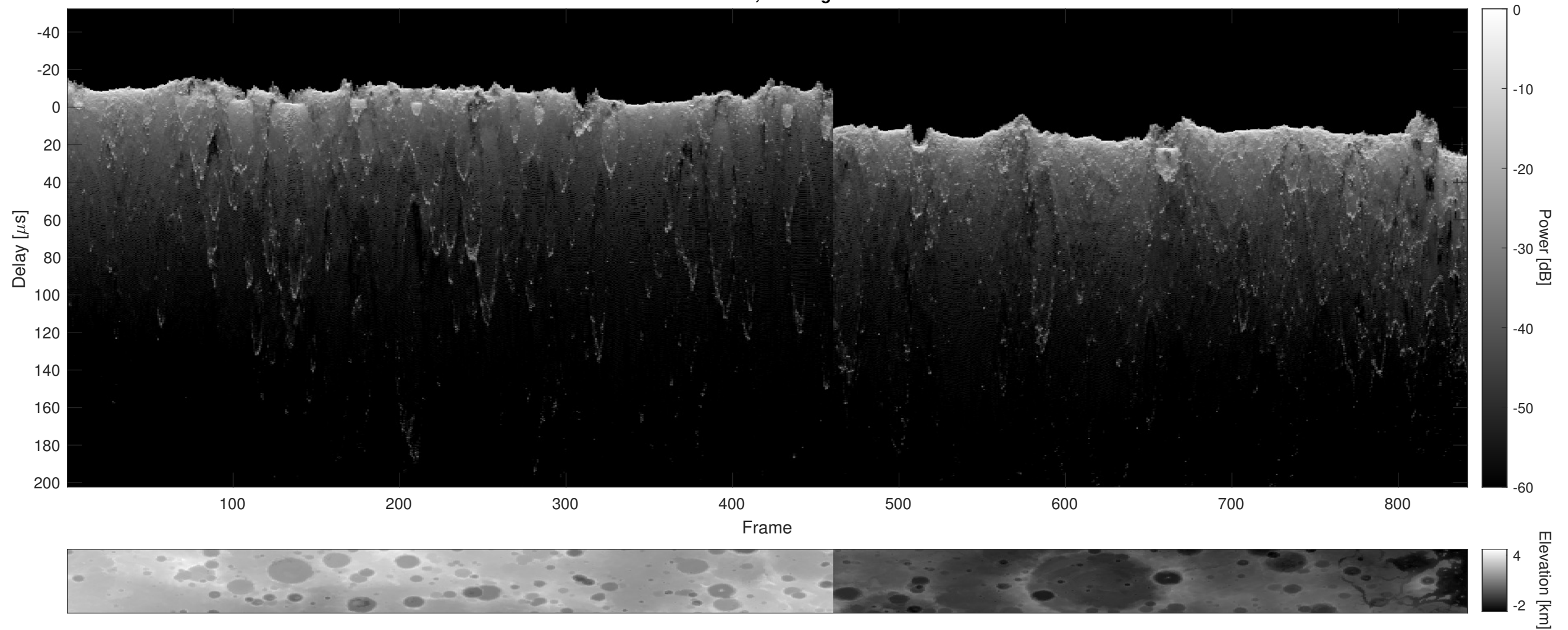
Orbit 6186, Cluttergram
