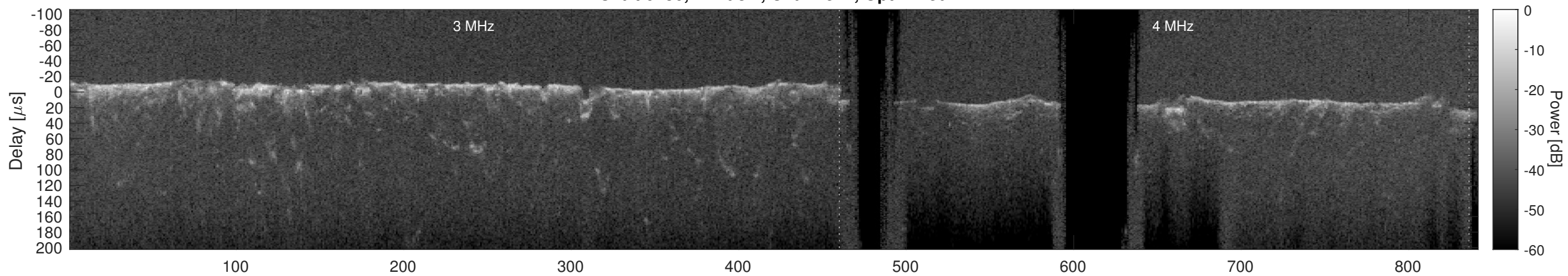
Orbit 6186, Cluttergram
