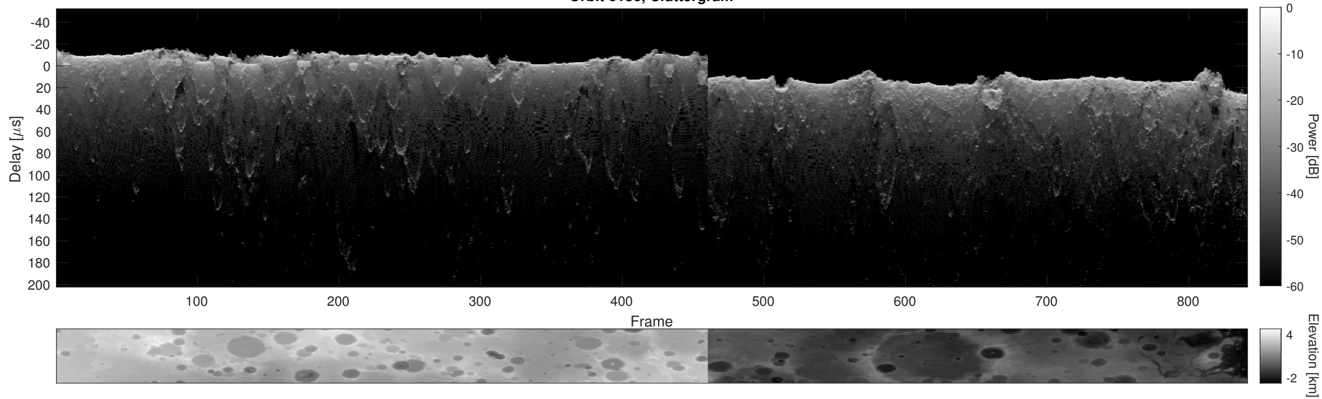
Orbit 6186, Cluttergram
