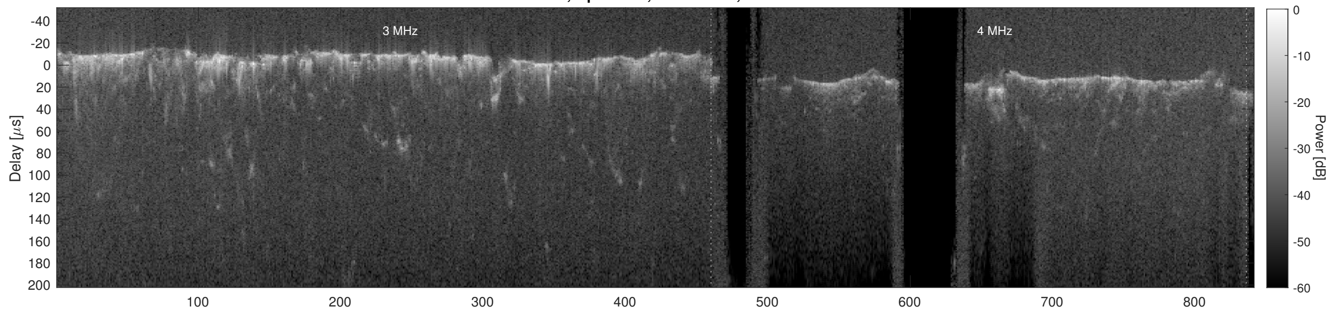
Orbit 6186, Cluttergram
