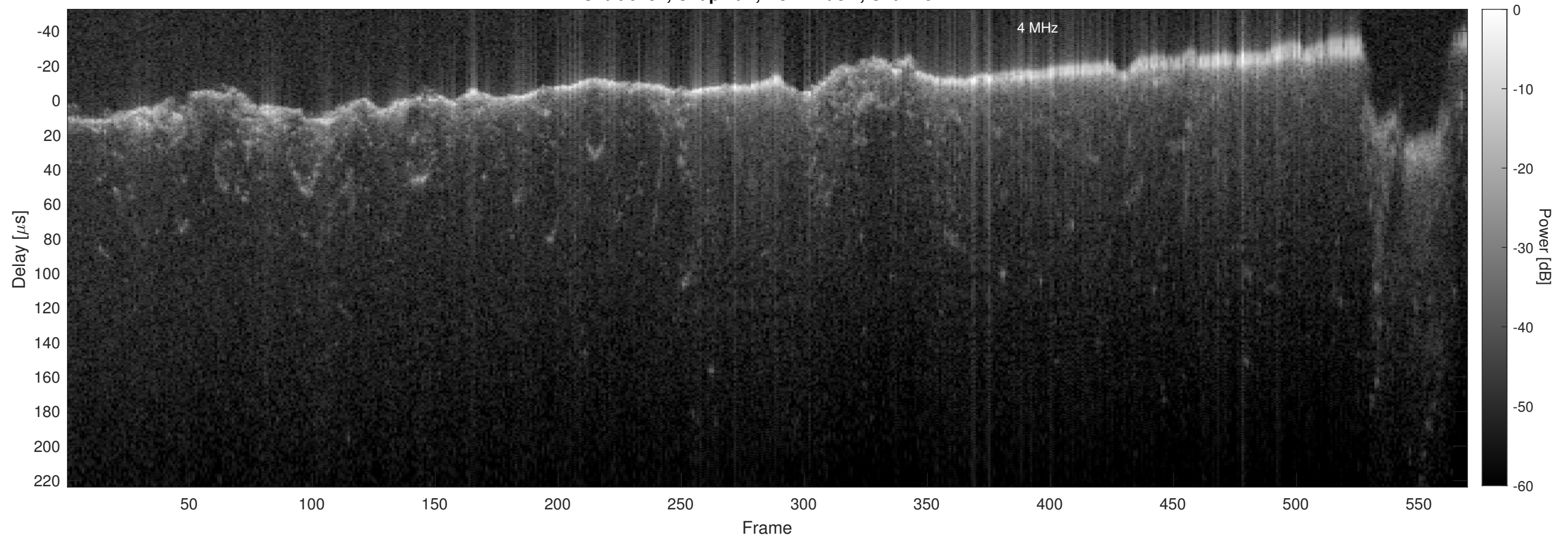
Orbit 6187, Chapman, No Window, Channel 2
