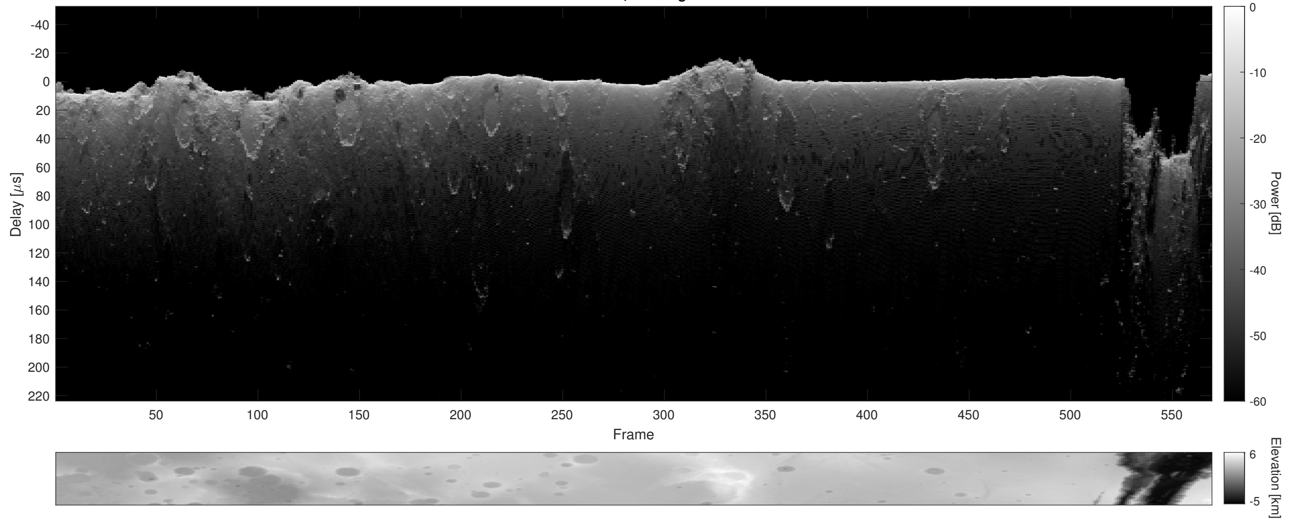
Orbit 6187, Cluttergram
