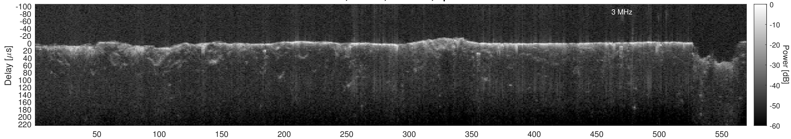
Orbit 6187, Cluttergram
