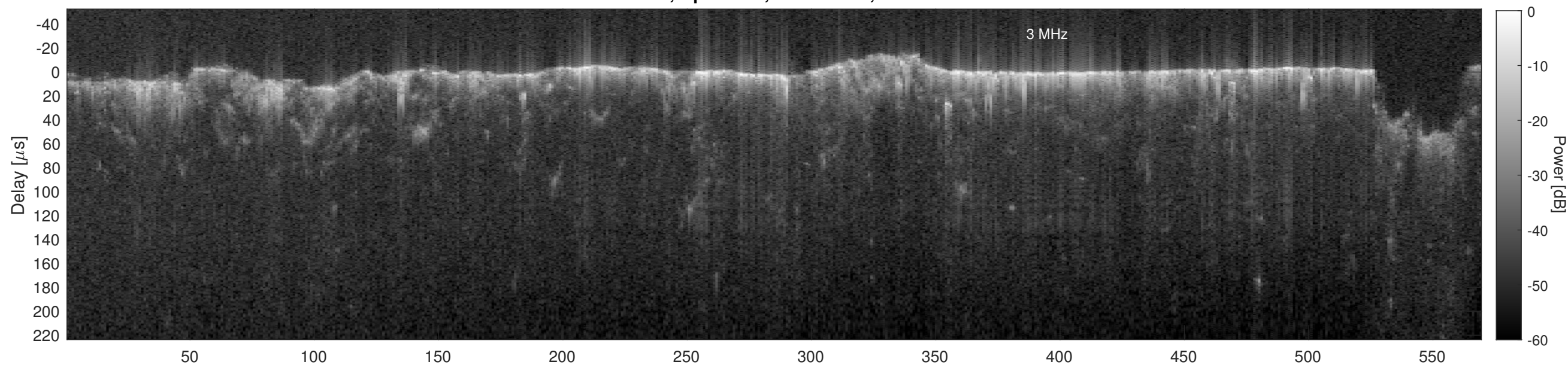
Orbit 6187, Cluttergram
