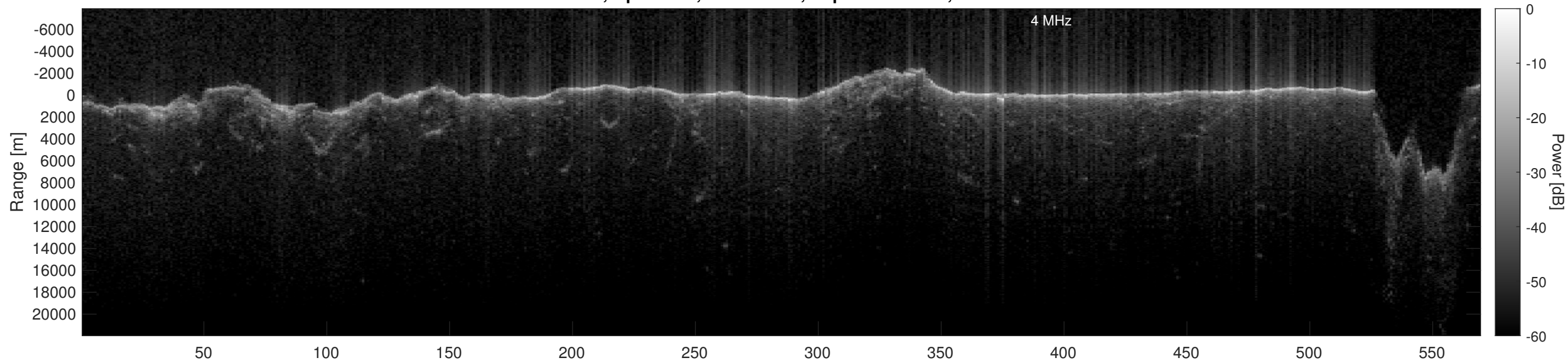
Orbit 6187, Optimized, No Window, Depth-Corrected, Channel 2
