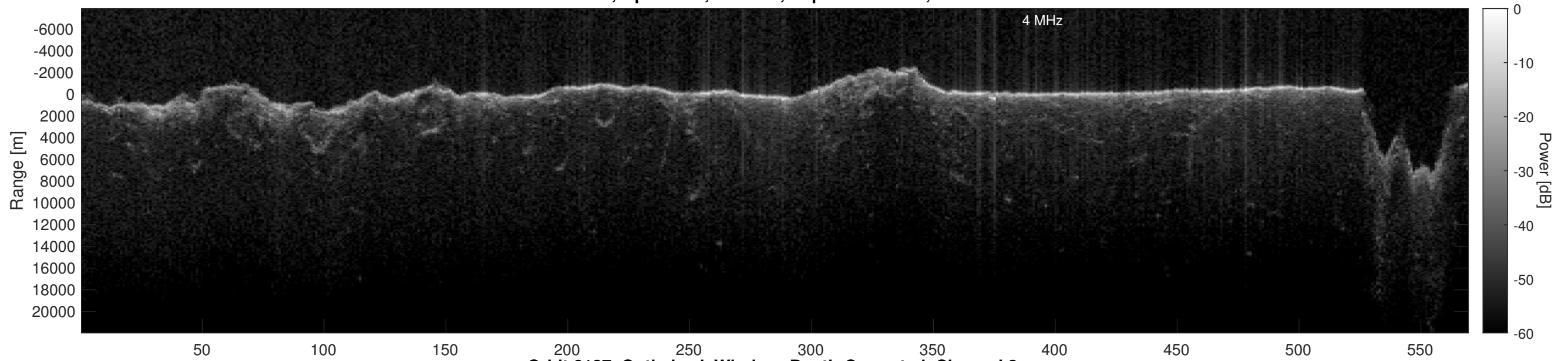
Orbit 6187, Optimized, Window, Depth-Corrected, Channel 2
