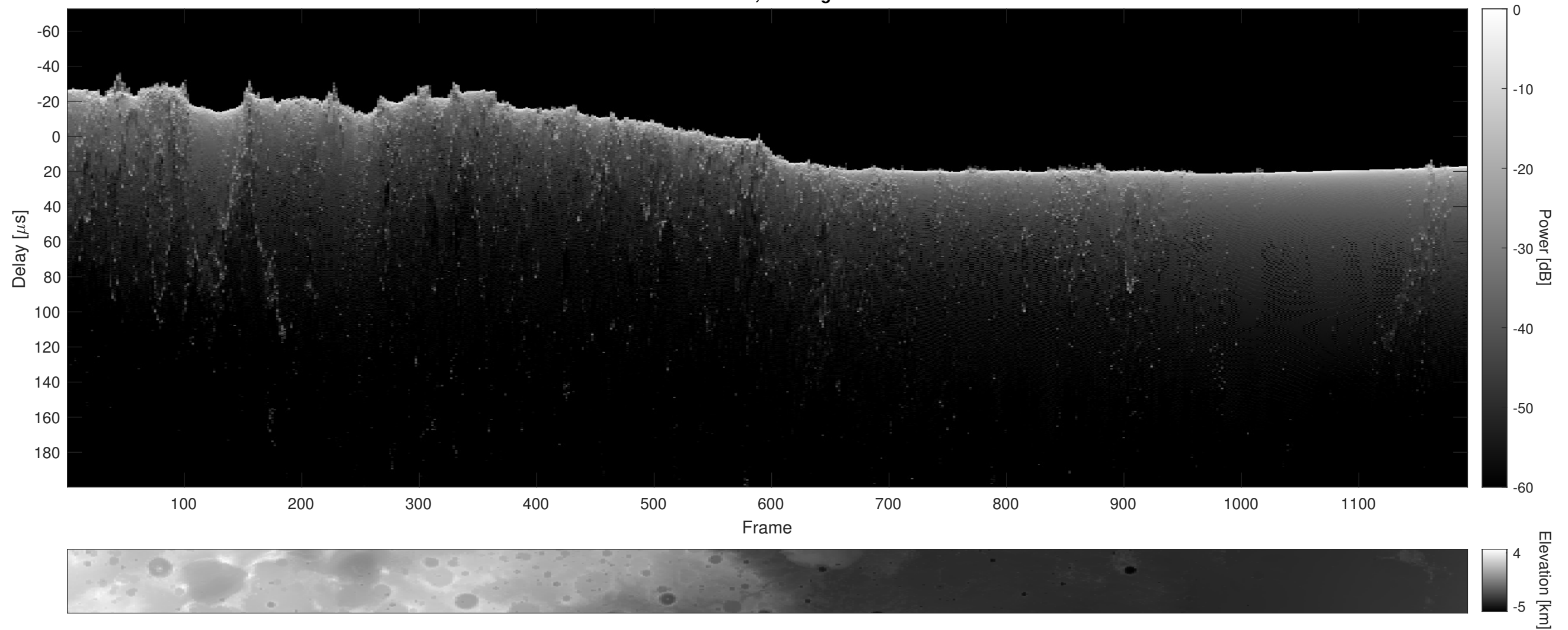
Orbit 6188, Cluttergram
