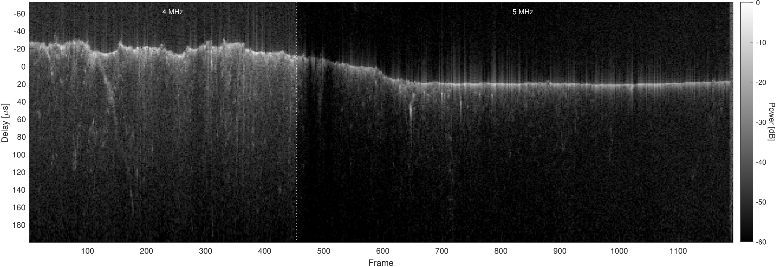
Orbit 6188, Optimized, No Window, Channel 2
