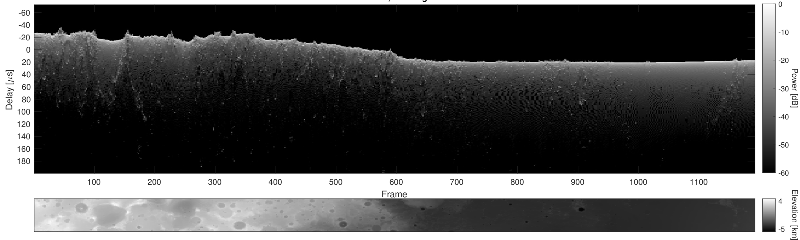
Orbit 6188, Cluttergram
