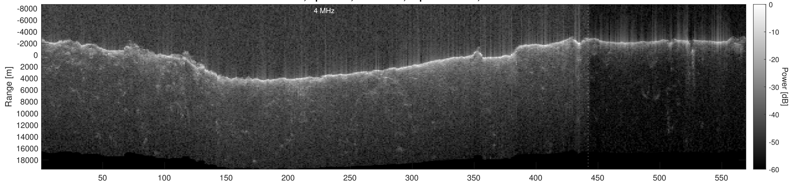
Orbit 6189, Optimized, No Window, Depth-Corrected, Channel 2
