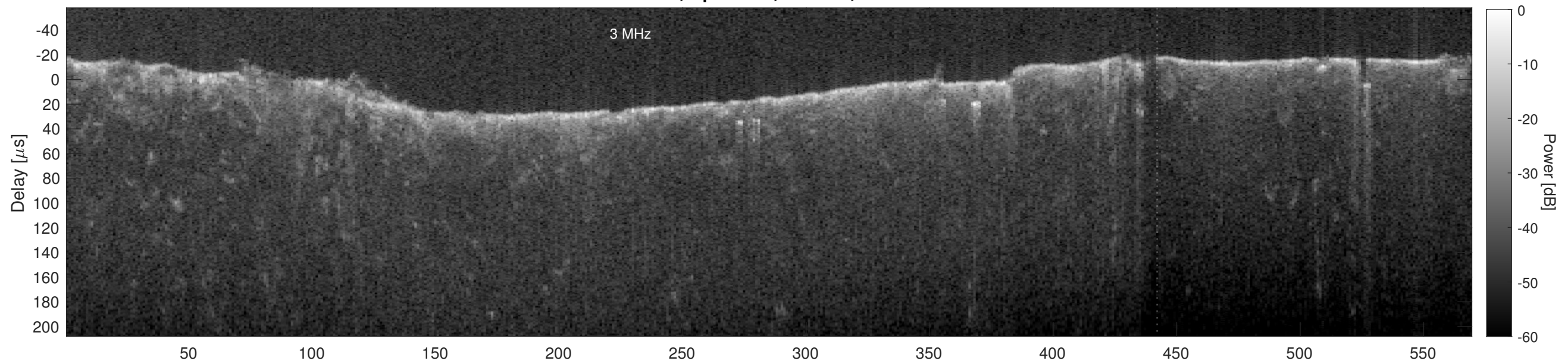
Orbit 6189, Cluttergram
