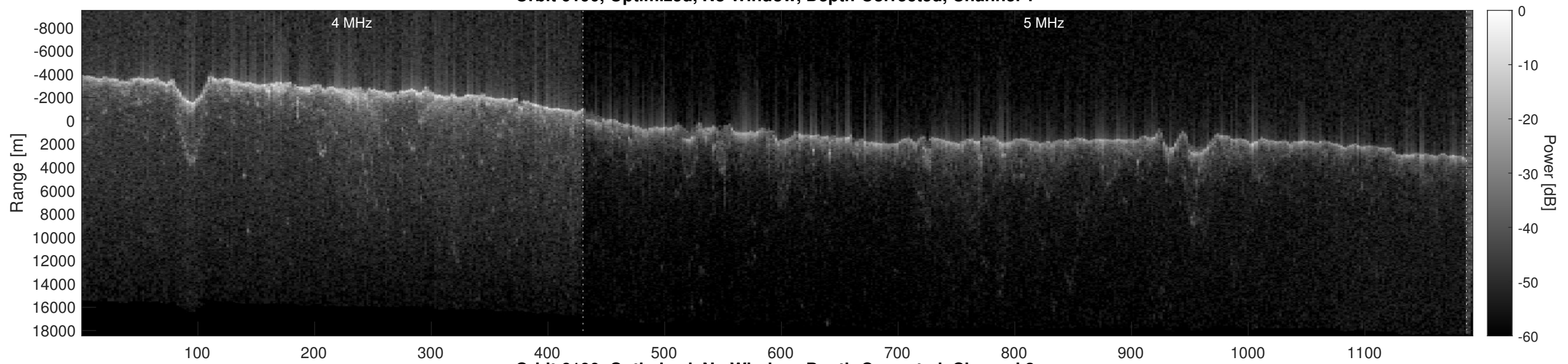
Orbit 6190, Optimized, No Window, Depth-Corrected, Channel 2
