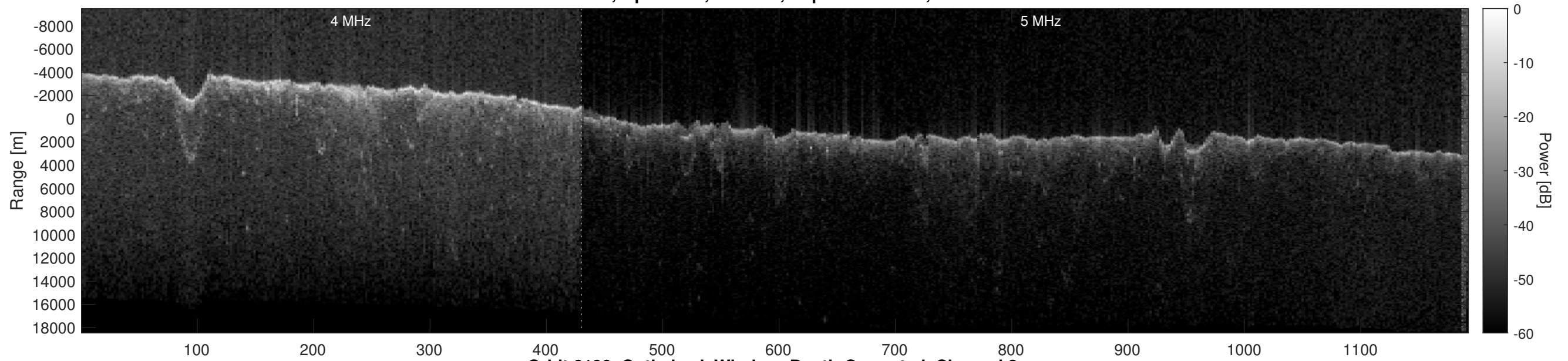
Orbit 6190, Optimized, Window, Depth-Corrected, Channel 2
