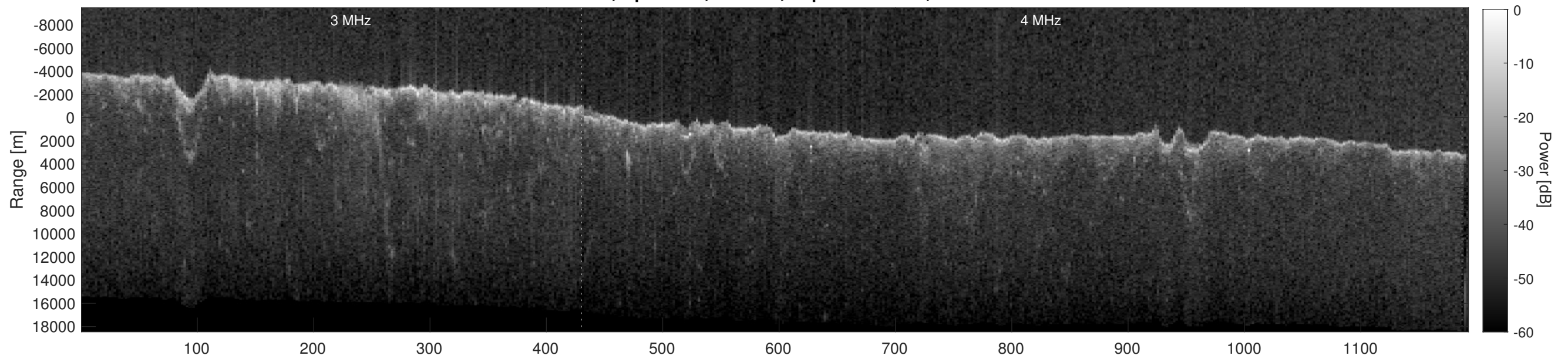
Orbit 6190, Depth-Corrected Cluttergram
