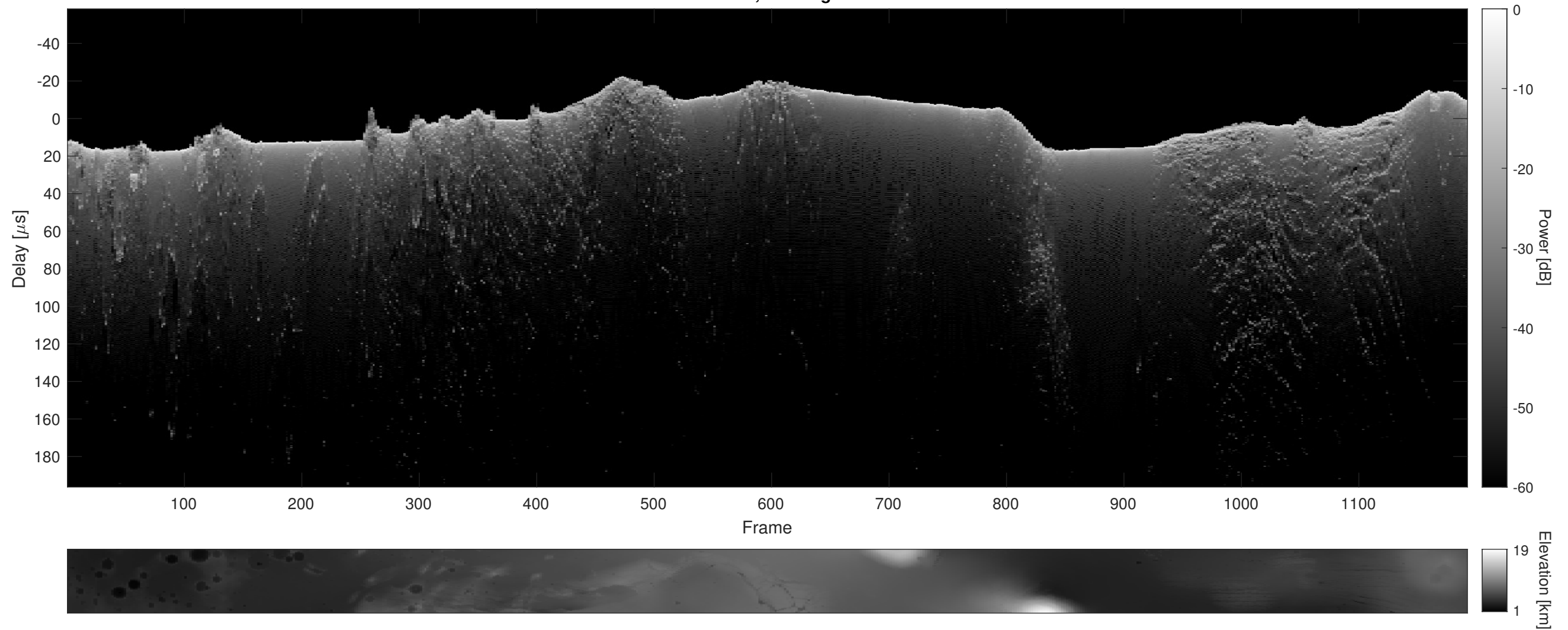
Orbit 6191, Cluttergram
