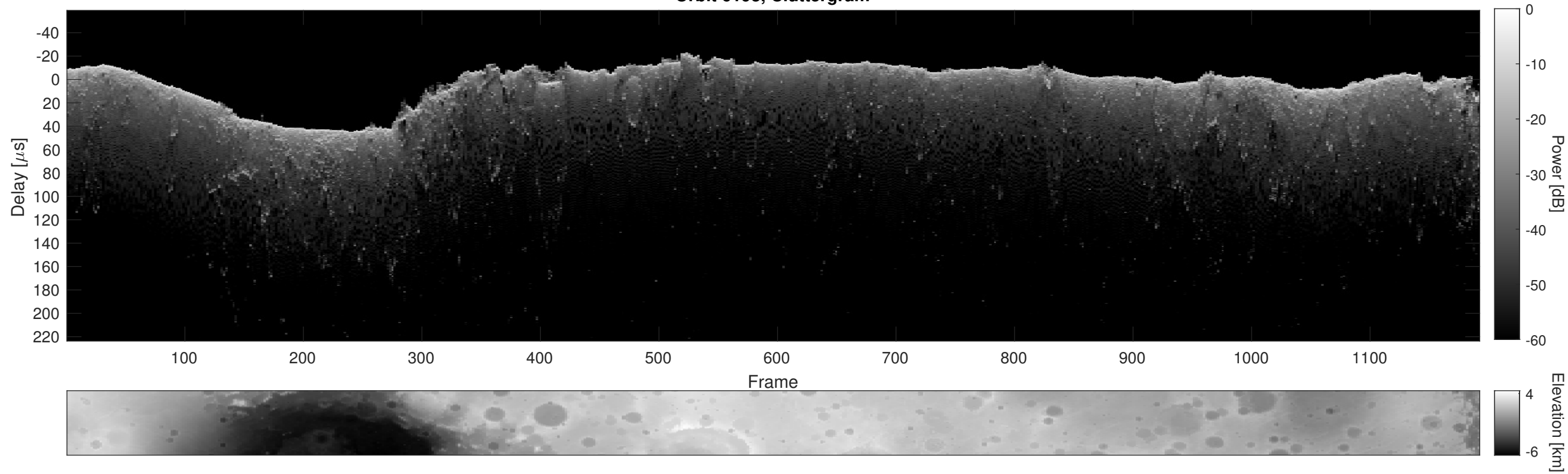
Orbit 6193, Cluttergram
