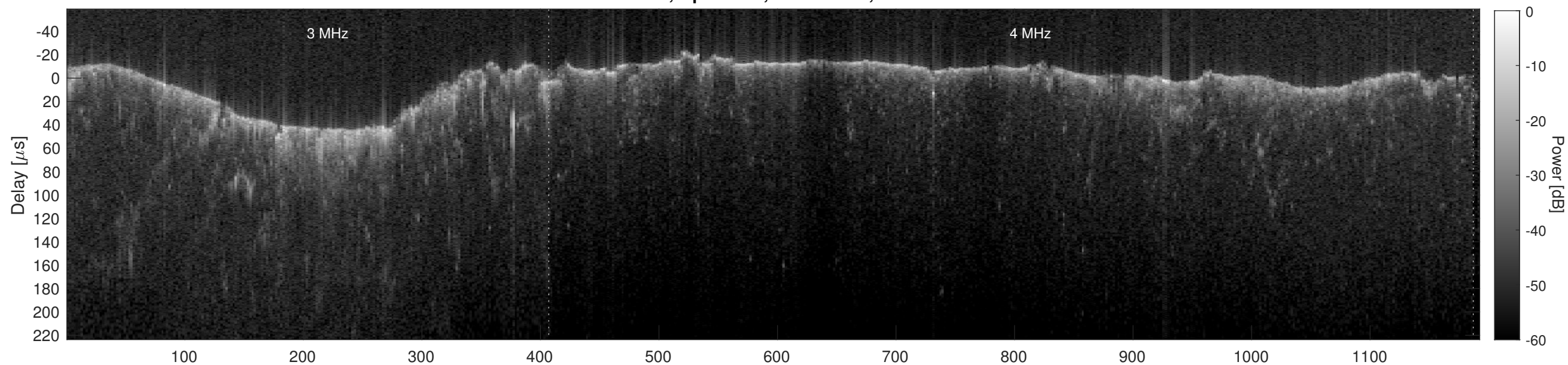
Orbit 6193, Cluttergram
