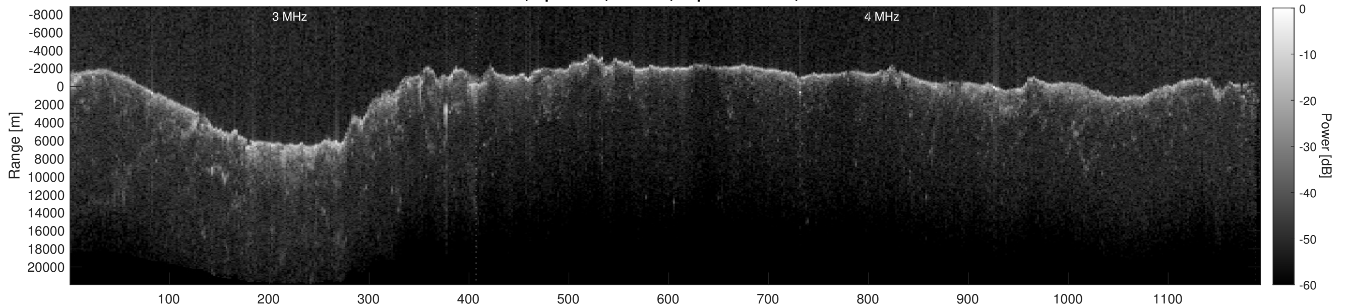
Orbit 6193, Depth-Corrected Cluttergram
