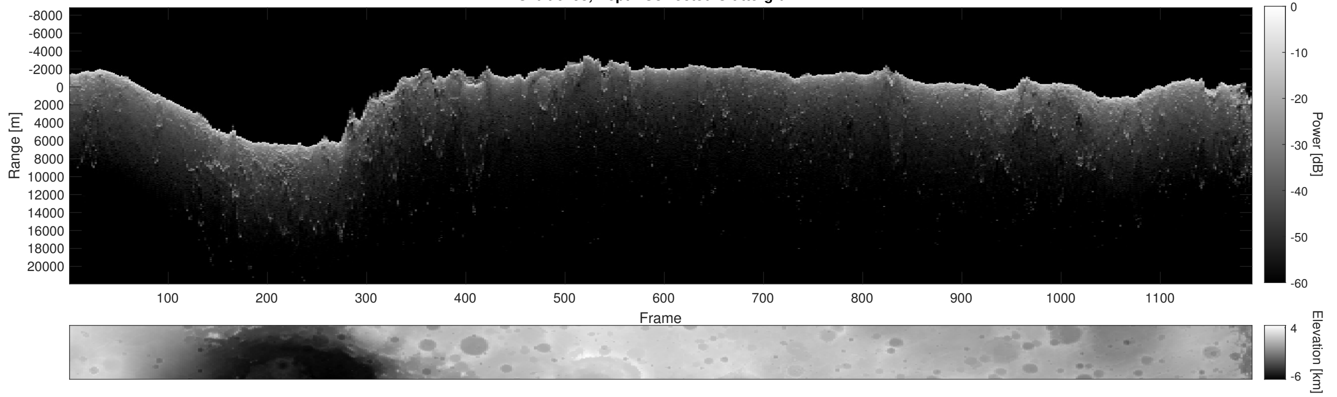
Orbit 6193, Depth-Corrected Cluttergram
